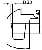
DETAIL C SCALE 3.000
